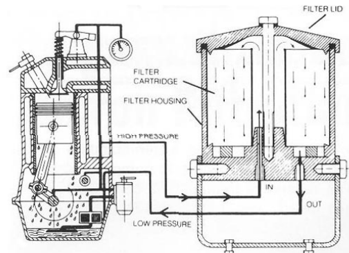
THE KLEENOIL FILTER CARTRIDGE
